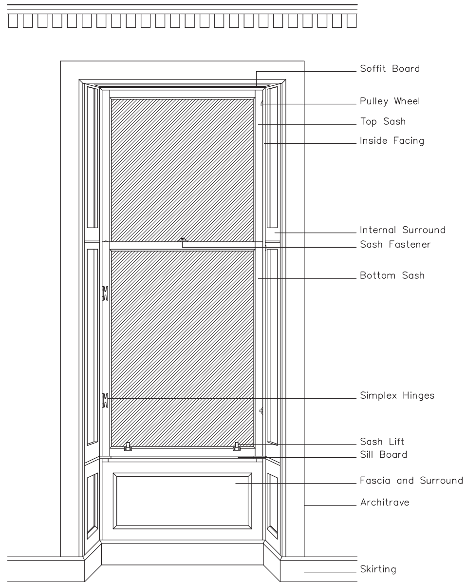
Timber Sash and Case Window – Internal Elevation.
