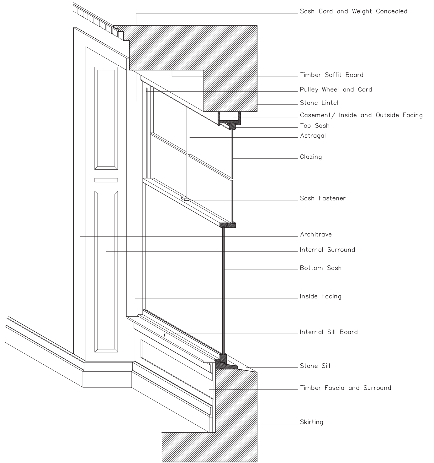
Timber Sash and Case Window – Isometric Projection.
